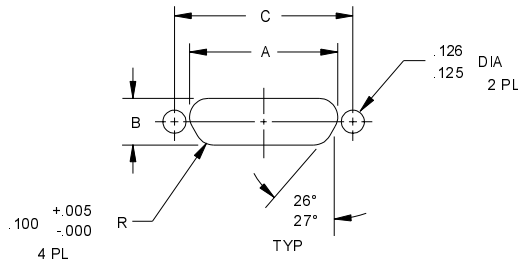
SIZES 9-69 REAR PANEL CUTOUT FOR PLUG & RECEPTACLE METAL
