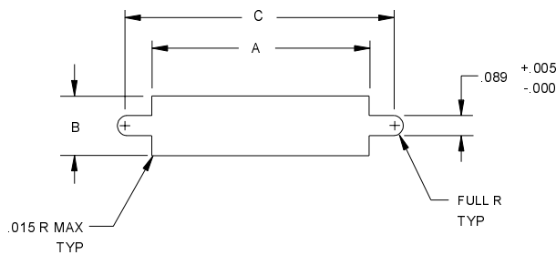
SIZE 9-69 FRONT PANEL CUTOUT FOR PLUG & RECEPTACLE METAL
